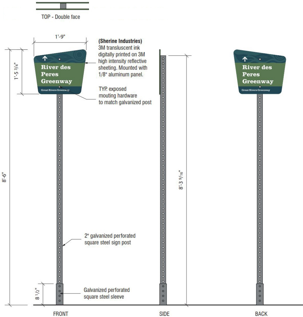
1 FRONT ELEVATION - SIGN FACE LAYOUT 3/4" = 1'-0"
